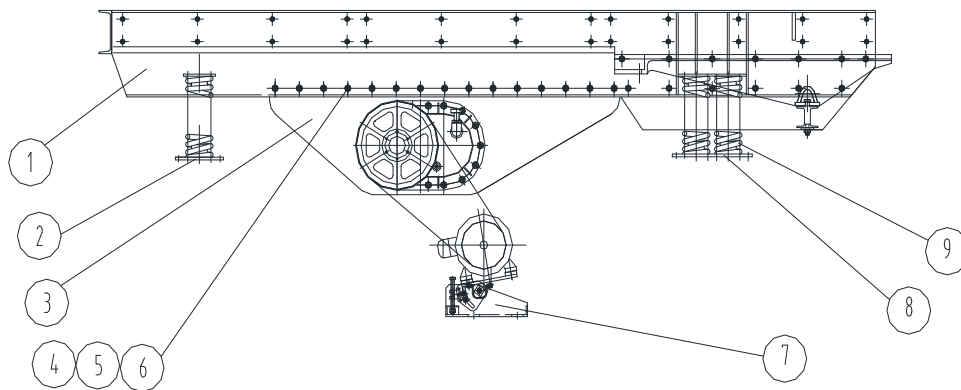
TF4016 Vibrating Feeder Assembly
